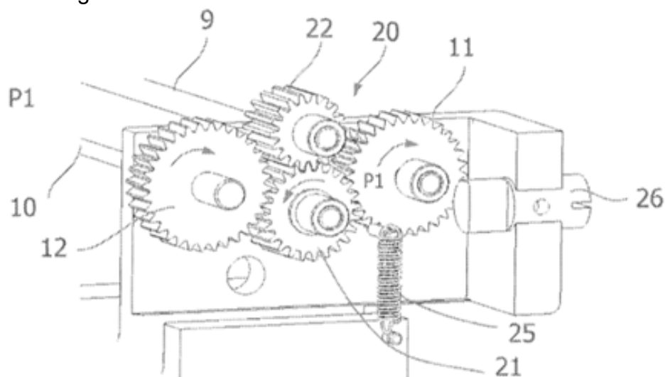
1b. Forward gear
