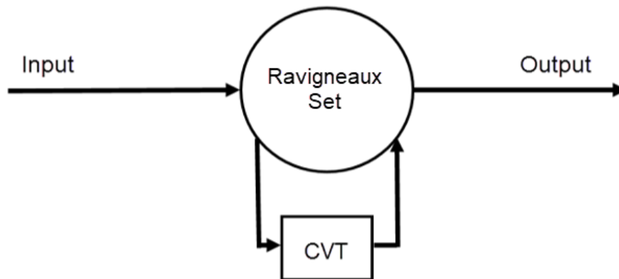
Figure 1 illustrates a power-split transmission including a combination of a summing/distributing Ravigneaux set and a CVT. Both the input and output of the CVT are connected to the summing/distributing Ravigneaux set. Torque from the input shaft is divided at the Ravigneaux set, summed at the Ravigneaux set, and output to the output shaft.
