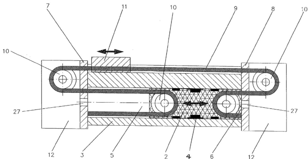
Figure 2 illustrates a transmission including piston (2) and output (11). Piston (2) provides input to belt (9) by movement back and forth in cylinder (3). Belt (9) engages rollers (10) and is connected to output (11), such that movement of the piston (2) is doubled at output (11).
