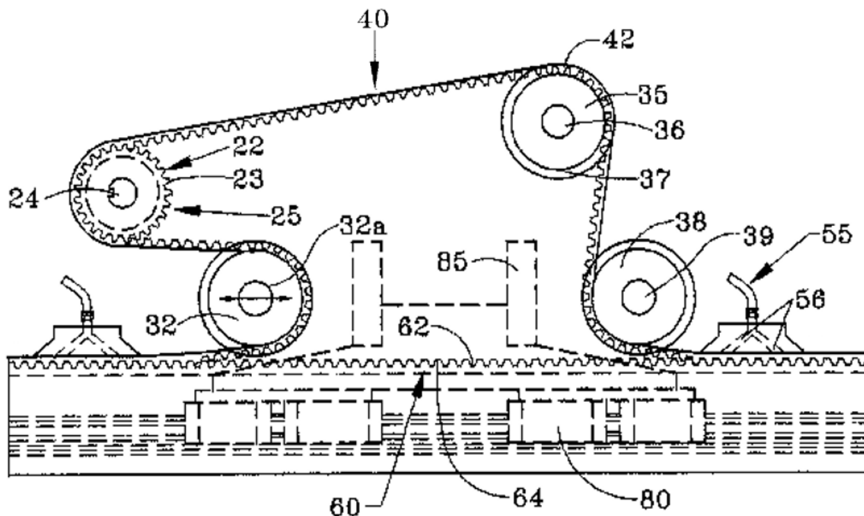
Figure 2 illustrates a transmission including rotary input (24) and output toothed rack (60). Input (24) drives belt (40) which engages toothed rack (60).
