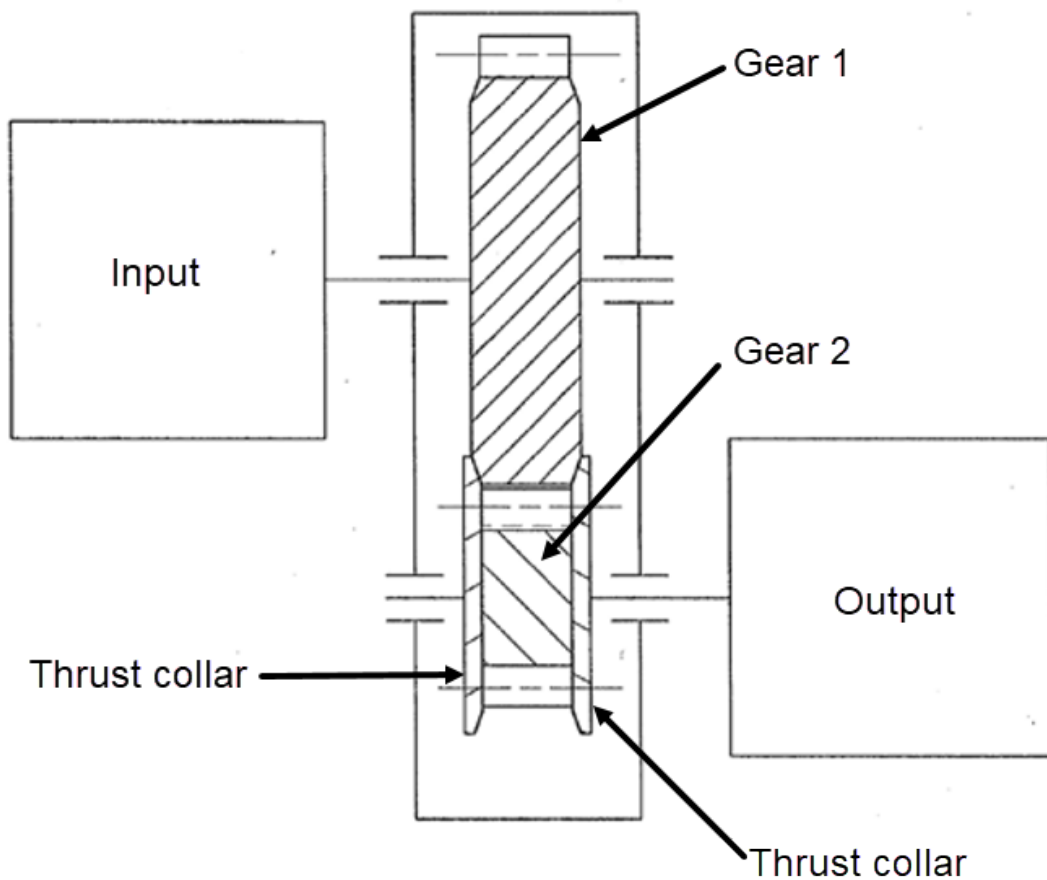
Figure 1 illustrates a pair of toothed spur gears (1) and (2) positioned relative to each other using left and right thrust collars attached to the surface of gear (2). The thrust collars are regarded as comprising specially adapted surfaces on the gears by which the two spur gears are positioned relative to one another.
