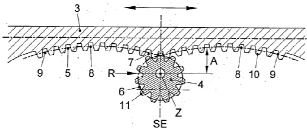
Figure 2 illustrates a rack and pinion gearing having a pinion (4) which is eccentrically mounted.
